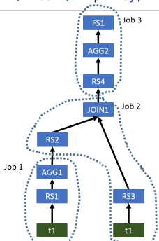
Source: The original operator tree [23]
