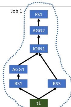
Source: The optimized operator tree [23]
